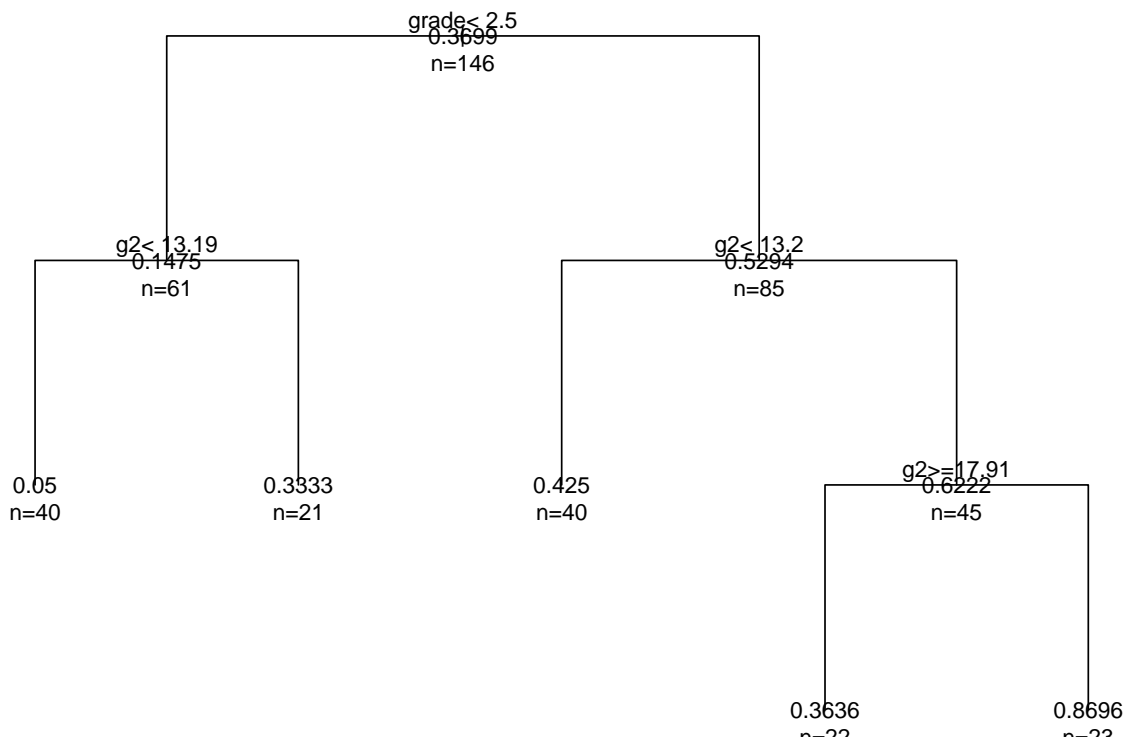
Figure 13: plot(fit, uniform = TRUE); text(fit,use.n = TRUE,all = TRUE)
