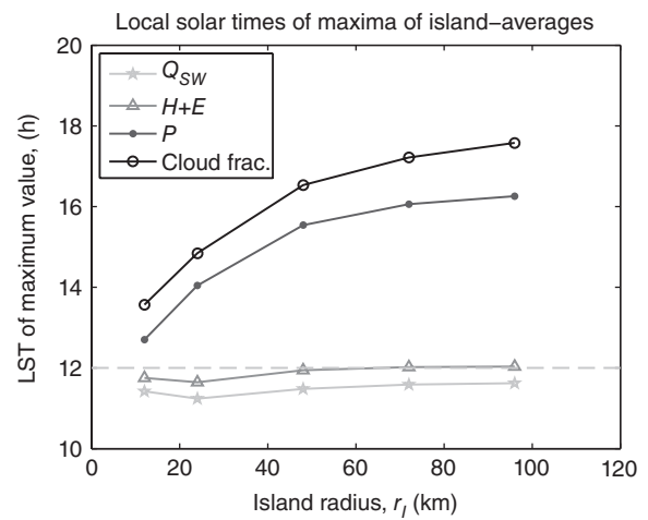
Figure 15. As Figure 5; plot of phases of the maxima of island-averaged surface solar radiation Q_{SW} (stars), surface enthalpy fluxes H + E (triangles), precipitation P (dots), and cloud fraction (open circles) against island radius, for a set of simulations with SAM with a reduced island surface heat capacity.
