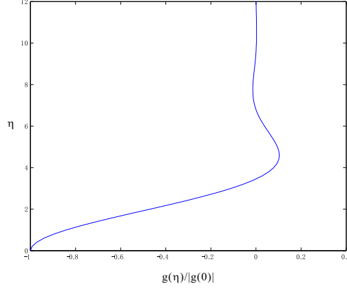
Figure 2.8.1: Velocity profile of a 2D slow flow into a line sink in a density-stratified fluid. Calculations by G. D. Lee, 2002. The abscissa is f'(\eta)/|f'(0)| = g(\eta)/|g(0)| . The ordinate is \eta = z(c/x)^{1/4} .
