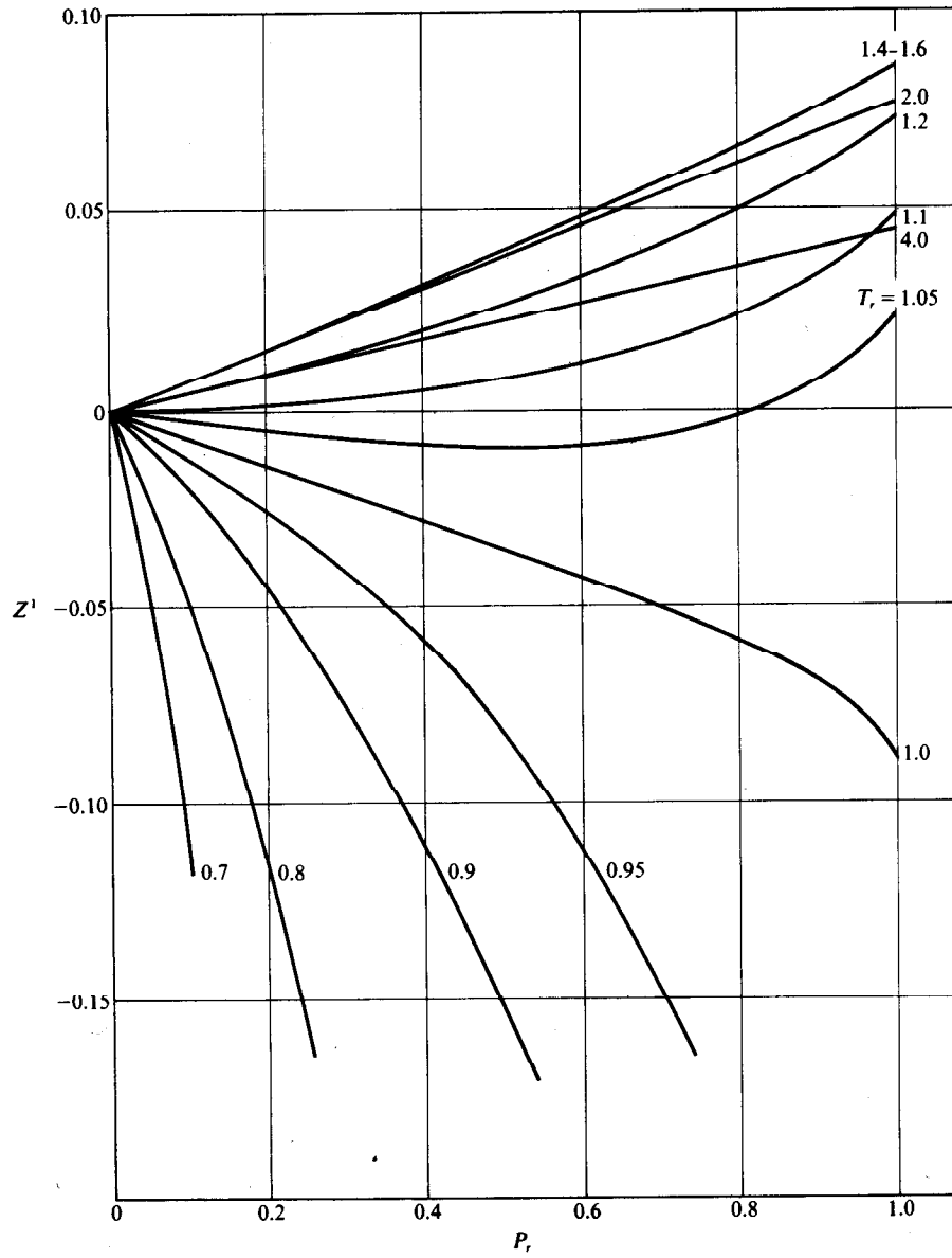
Figure 3.14 Generalized correlation for Z' , P, < 1.0 . (Based on data of B. I. Lee and M. G. Kesler, ibid. )
