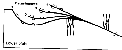
Fig. 11. Development of a basement culmination means that the master detachment faults become progressively more bowed. A new detachment fault propagates from the culmination, as it becomes more accentuated. This fault in turn also becomes bowed upward. A succession of progressively less bowed detachment faults results (sequence of 1-4). Each new detachment fault bites further into the lower portions of the upper plate, and excises more and more of the stratigraphic section. Attempts to restore the cross-section using the technique of balanced cross-sections will fail, unless the phenomenon of multiple detachment can be properly accounted for. Cross-sections cannot be balanced using only the youngest of the detachment faults. Displacement of a hypothetical dike swarm is shown schematically.
