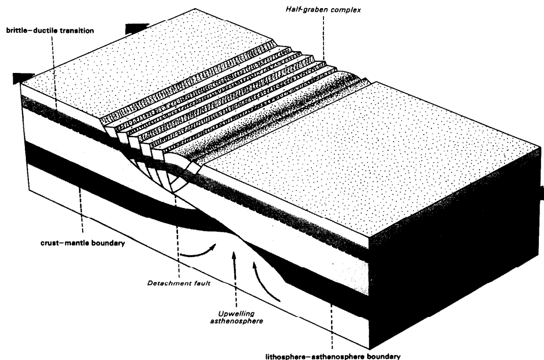
Fig. 6. Extension of the continental crust using a single lithospheric dislocation, after a model presented by Brian Wernicke at the Geological Society of America convention at Salt Lake City in 1983. The detachment fault represents the upper levels of a shallow-dipping shear zone that passes all the way through the lithosphere.
