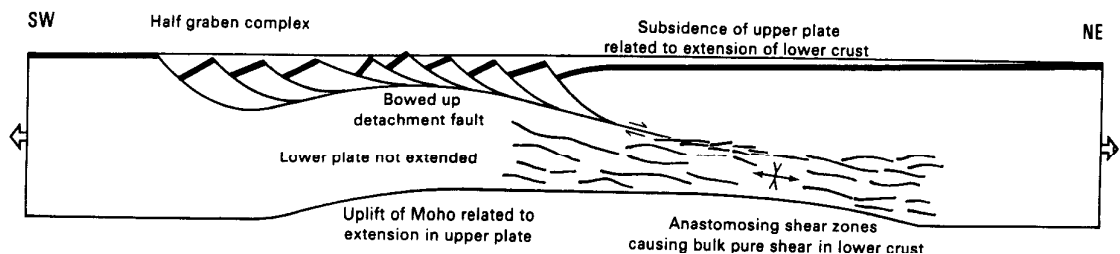
Fig. 8. Model of detachment of the upper crust during horizontal extension, involving a shallow-dipping detachment fault which disappears with depth into a ductile shear zone. The lower crust, however, is subject to pure shear at the termination of the movement zone. Uplift of the crust-mantle boundary is caused by a combination of bowing upward of the (undeformed) lower plate (dominant in the west), and the results of ductile attenuation of the lower part of the lithosphere (dominant in the east).
