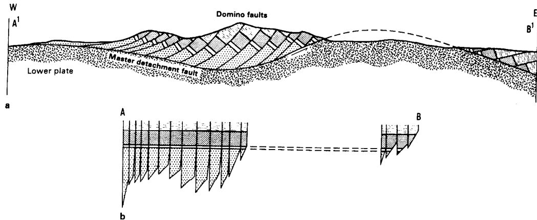
Fig. 13. A (schematic) cross-section produced as the result of multiple listric normal faulting and excisement (a). Restoring this section to the undeformed state (b) shows that segments of the upper plate are missing. Note that the detachment fault roots to the west, not to the east. Detachment faults are often rotated as the result of asymmetric uplift as the result of the formation of basement culminations.
