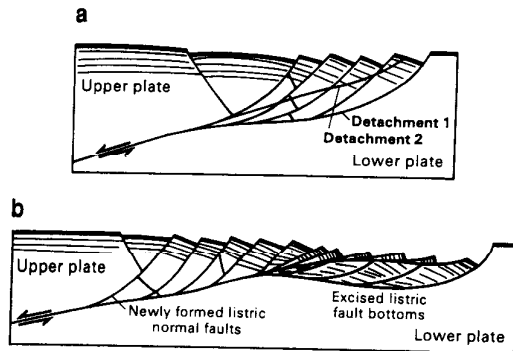
Fig. 14. Multiple detachment leads to excisement of listric fault bottoms. Diagram (a) shows a major splay that has branched from the previously active detachment fault. In (b) this splay has become the master detachment, and excisement of the lower portion of the upper plate has occurred. Previously active normal faults are abruptly terminated at the younger detachment. Younger listric normal faults have formed, associated with the new detachment surface. Multiple detachment thus explains the abruptly truncated, relatively planar, steeper normal faults of the upper plate.
