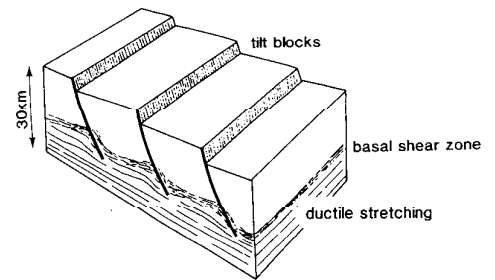
Fig. 4. Seismological observations tell us that the continental crust extends now as the result of arrays of steeply-dipping, deeply-biting normal faults. Crustal-scale rotating tilt blocks are bounded at depth by ductile shear zones that relax stresses built up around the base of a normal fault after a seismic rupture. The shear zones must be shallow dipping to accommodate strain incompatibilities between the ductilely stretching lower crust and the brittlely extending upper crust.
