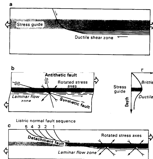
Fig. 19. (a) Extension of the stress guide defined by the brittle-ductile transition results in the formation of a through-going fault. Continued extension results in a sub-horizontal shear zone allowing detachment of the middle to lower continental crust at some depth below the brittle-ductile transition. This sets the stress axes over a wide area into inclined attitudes (ideally 45^\circ to the horizontal). (b) The Coulomb-Mohr solutions for the synthetic failure plane favour the formation and propagation of a low-angle normal fault. (c) This acts as a master fault at depth, from which splay successive listric normal faults (1-5) which extend its area by progressively eating into the footwall of the previously formed fault.
