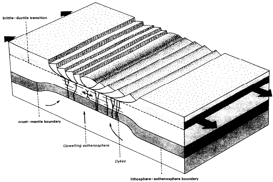
Fig. 2. Three-dimensional illustration of the symmetric pure shear model for continental extension. The detachment fault is seen as representing an ancient brittle-ductile transition in the Earth's crust. Brittle deformation in the upper plate is synchronous with ductile deformation in the underlying lower plate, which is the result of bulk coaxial extension as the entire lower part of the lithosphere uniformly stretches.
