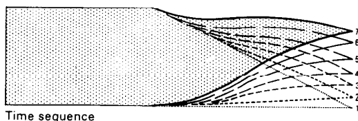
Fig. 10. Schematic illustration of the progressive uplift of a lithospheric wedge as the load exerted by the upper plate is slowly removed, assuming zero flexural rigidity.
