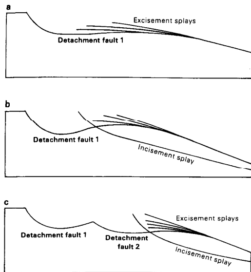
Fig. 18. Development of incisement-excise structures as the lower plate bows upwards. Excise faults splay from the currently active master detachment fault (a). Incisement of the detachment fault into the lower plate then follows, and new excise faults splay off the developing culmination (b). In this way, as the result of successive incisement-excise sequences, relatively deep levels of the lower plate can be exposed.
