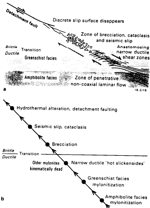
Fig. 9. The concept of an evolving shear zone implies spatial and temporal variation. Diagram (a) shows the spatial variation of material behavioural fields expected with increasing depth, with detachment faults disappearing into zones of brecciation, cataclasis and seismic slip, and then passing into ductile shear zones. A rock transported upwards in the footwall of a detachment fault transposes the spatial sequence of material behavioural fields in (a) into a time sequence of material response (b).
