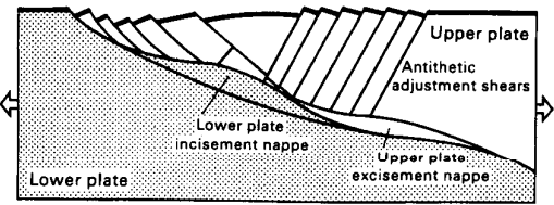
Fig. 16. Splays in the detachment fault lead to the formation of multiple detachment surfaces. Incisement nappes form when the detachment bites into the lower plate, and excisement nappes when the detachment slices off a portion of the lower part of the upper plate. Shaded portion of figure indicates original lower plate.
