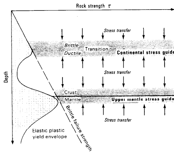
Fig. 3. Depth-dependent rheology of the continental crust, assuming the concept of an elastic-perfectly plastic rheology (after Chen & Molnar 1983). The strength maximum around the depth at which the brittle-ductile transition takes place defines the continental stress guide.
