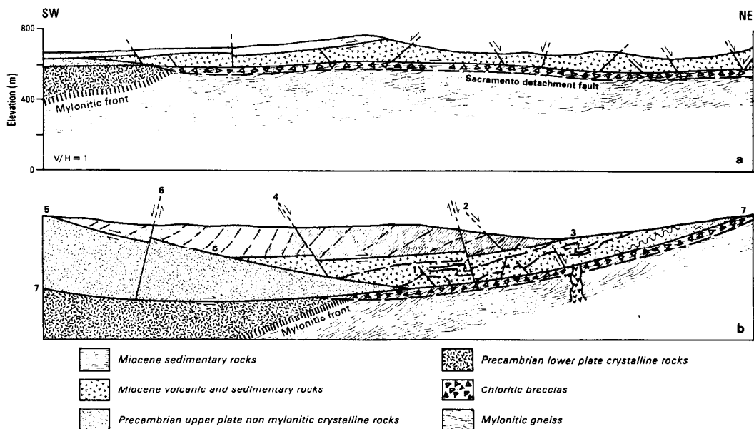
Fig. 17. Thin detachment slices in the upper plate of the southern Sacramento Mountains detachment fault (a), from McClelland (1984). Schematic cross-section (b) illustrates geological and geochronologic relations in this complexly deformed terrane. Three generations of detachment faults exist. The relative ages of high-angle and low-angle faults are indicated by numbers 1–7.
