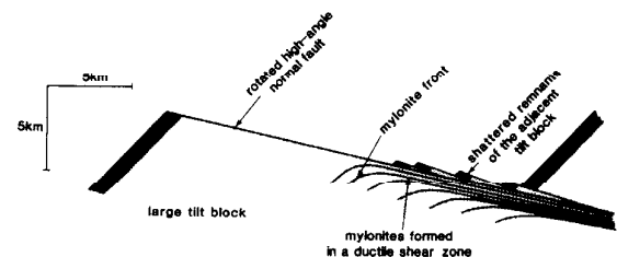
Fig. 5. One model for the origin of metamorphic core complexes is the domino-like rotation of crustal-scale tilt blocks. One such tilt block lying on its side would have many of the characteristics exhibited by a metamorphic core complex. The model supposes that the detachment fault is a rotated high-angle normal fault, but this requires a much larger variation in metamorphic grade along the crustal section thus exposed than is actually observed. (This is not the interpretation we propose. A more realistic model is shown in Fig. 20.)
