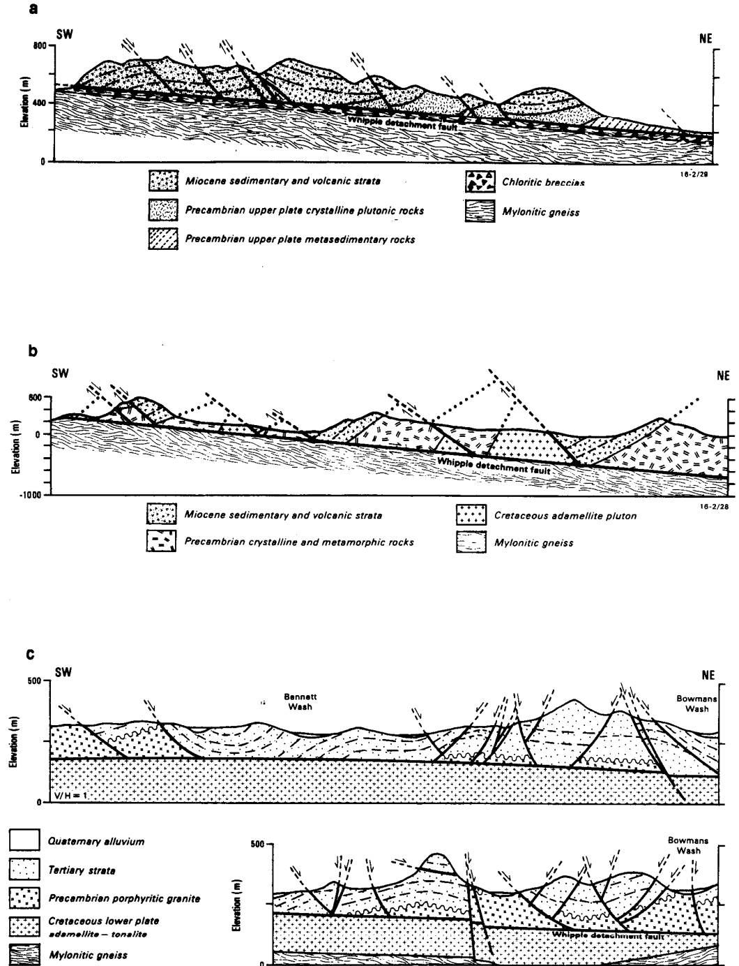
Fig. 12. Three cross-sections illustrating the wide variation in structural geometry of the upper plate rocks to the Whipple detachment fault. Each section shows the abrupt termination of upper plate structures at the detachment fault. The vertical and horizontal scales are identical. Cross-section (a) is through the upper plate of the Whipple detachment fault, in the eastern Whipple Mountains (adapted from Frost, in Anderson & Frost 1981). (b) is from Frost (1980) through the Whipple Wash canyon, eastern Whipple Mountains, where the geometry of upper plate faulting is well exposed. Numerous planar normal faults terminate abruptly at the main Whipple detachment fault. None of these faults cut the detachment. This suggests the present Whipple detachment fault is a relatively young feature. Cross-sections in (c) pass through the upper plate of the Whipple detachment fault, southern flank of the Whipple Mountains (from Thurn 1983). Tertiary strata are broadly folded, and offset by SW- and NE-dipping normal faults. Domino-style faulting cannot be invoked in this area, and Tertiary strata clearly have not been rotated in large tilt blocks and lowered onto the detachment fault. Once again, the cross-sections above the Whipple Fault cannot be balanced using presently visible faults, indicating that the Whipple Fault post-dates upper plate structure in this area, and that the detachment has excised the lower portions of the upper plate. See text for further information.
