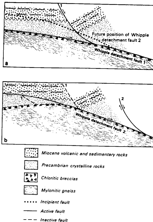
Fig. 15. Schematic representation of the time-evolution of the geometry of the Whipple detachment fault, to explain geological relations illustrated in Fig. 14. Section (a) illustrates inferred geometry of the Whipple Fault during phase 1 of its development. A listric normal fault (1) is associated with detachment fault 1. A splay is about to branch from this fault. Section (b) illustrates a subsequent phase of extensional deformation, where this splay (Whipple detachment fault 2) is now acting as the main detachment fault. This fault is also associated with a listric normal fault (2). However, the only indication that fault (1) in section (b) ever was a listric normal fault is the abrupt change in dip of strata that occurs across the fault.
