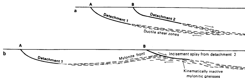
Fig. 21. Development of a mylonite front in the footwall of a younger detachment fault. The younger detachment fault transects mylonitic foliation. The mylonite front marks the location where the older mylonitic fabric in the exposed core complex rolls over, and diverges from the younger, capturing detachment fault.
