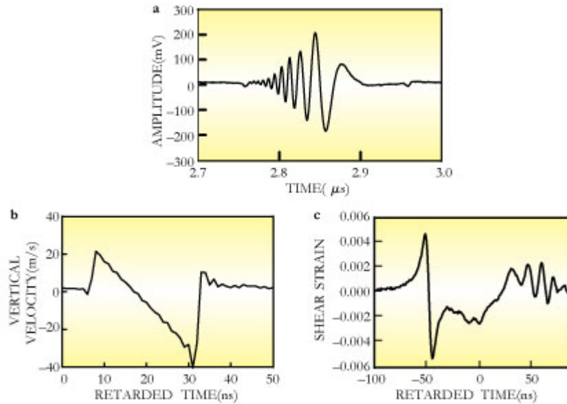
Figure 4: Shapes of SAW pulses.
