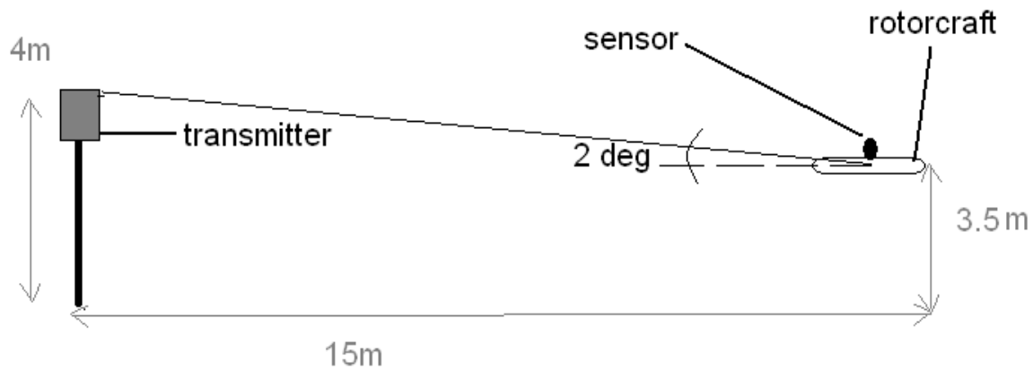
Figure 2: Transmitter location rationale
