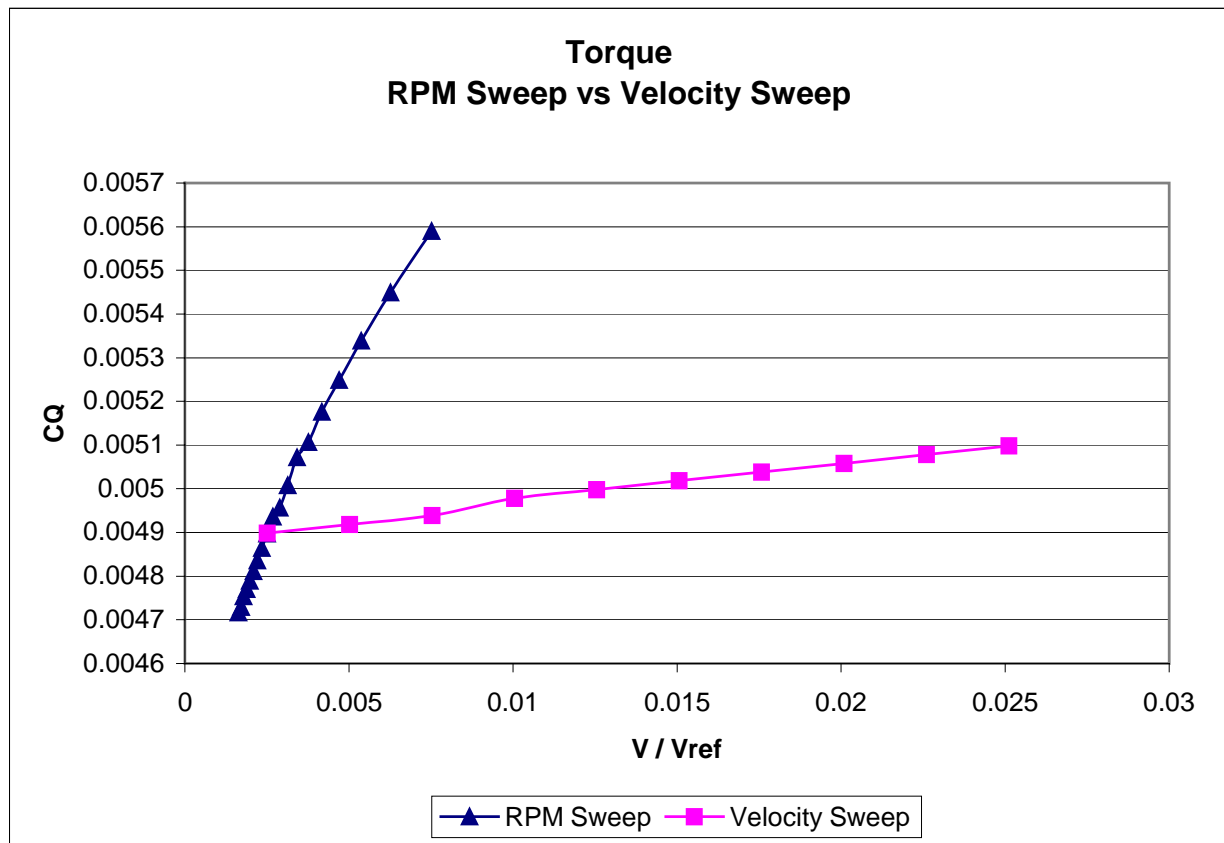
Figure 6: CQ vs. V/Vref
