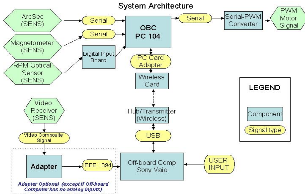
Figure 3: System Architecture
