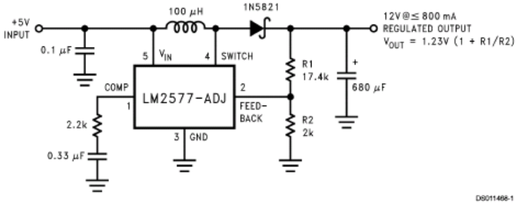
Figure 1: Setup of the Voltage Booster
