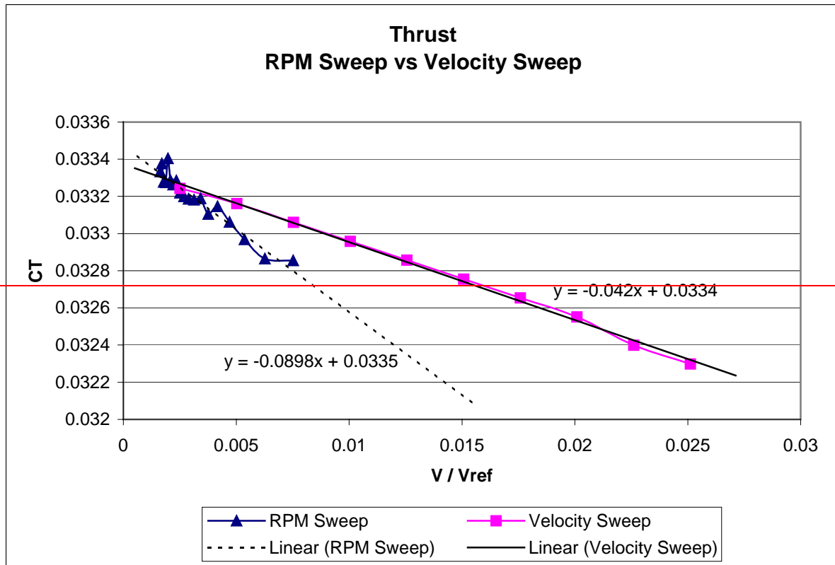
Figure 4: C_T vs. V/V_{ref}
