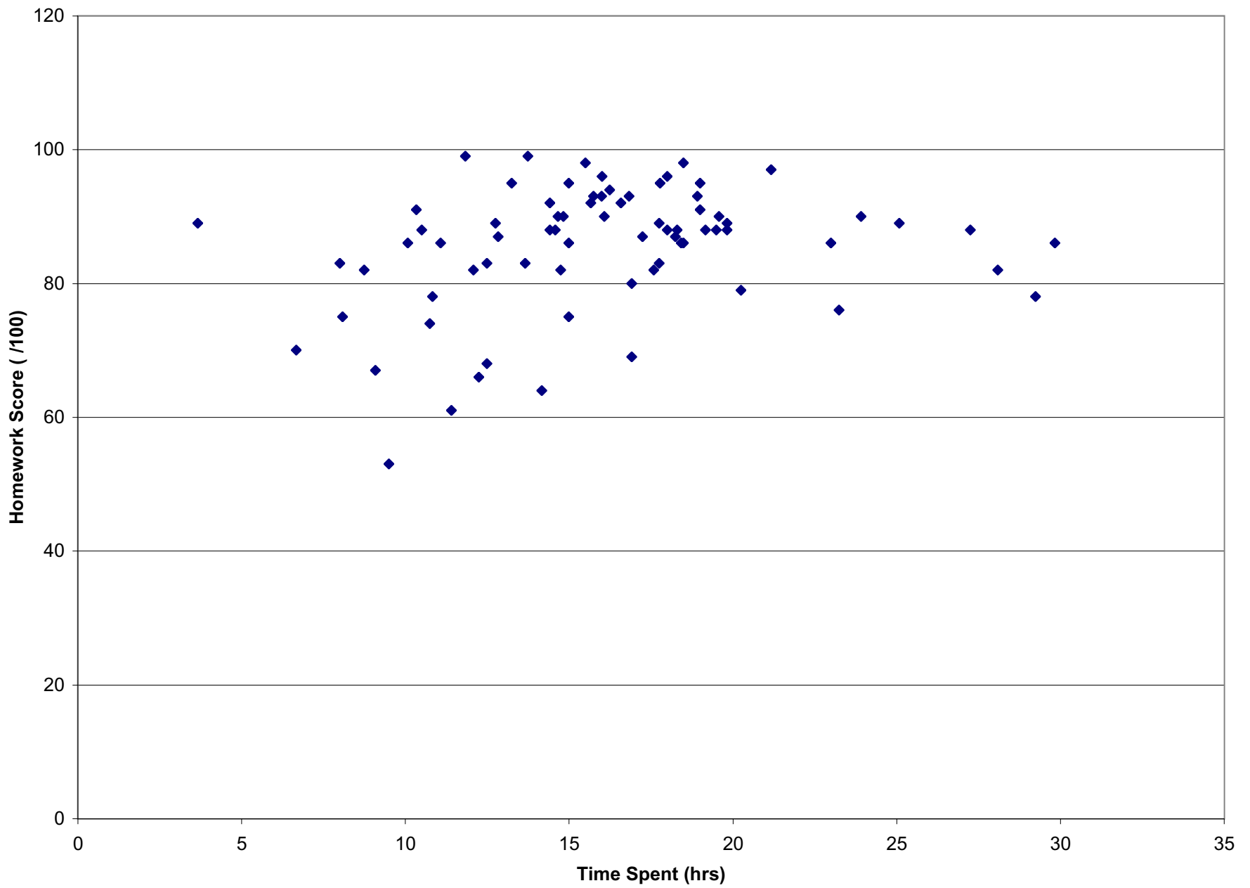
Time Spent vs. Homework Score
