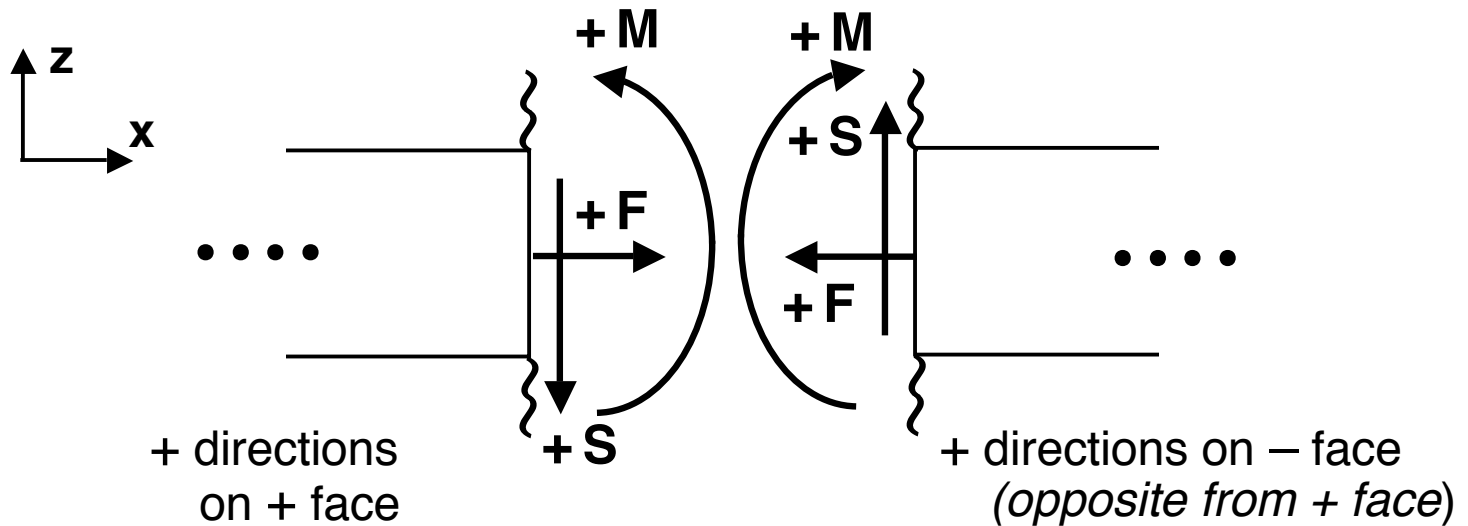
Figure M4.3-11 Overall aligned force system acting on cut faces of beam
