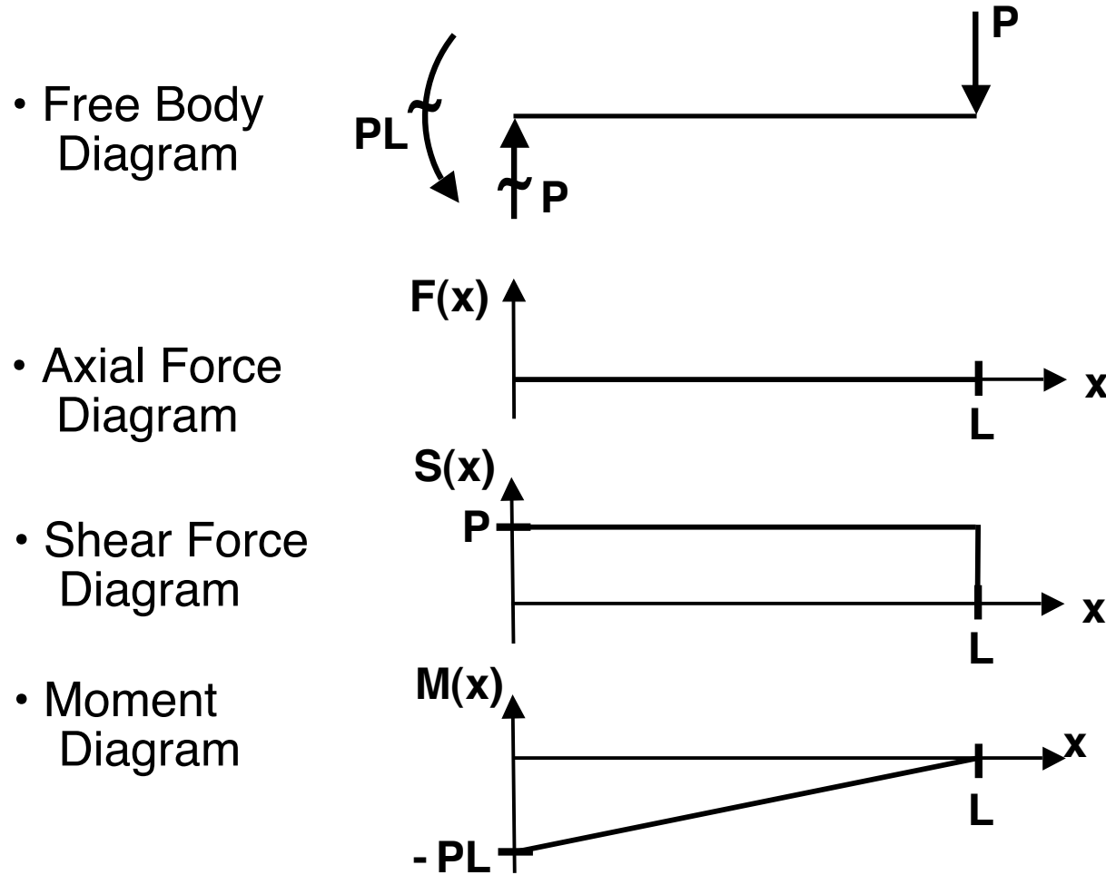
Figure M4.3-17 Force diagrams for cantilevered beam with tip load
