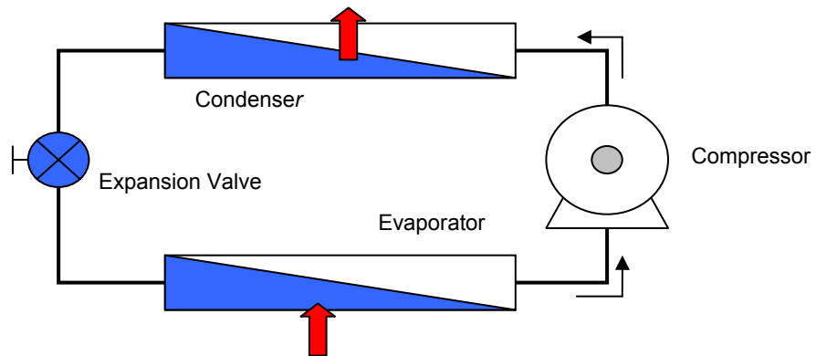
Figure 1 Refrigeration cycle
