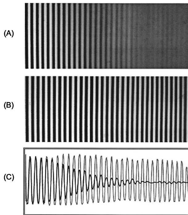
Fig. 4. Image of a bar pattern that was tilted at 60^\circ to the image plane. (A) Image from a conventional system, (B) image from a coded system after signal processing, and (C) traces through both images.
