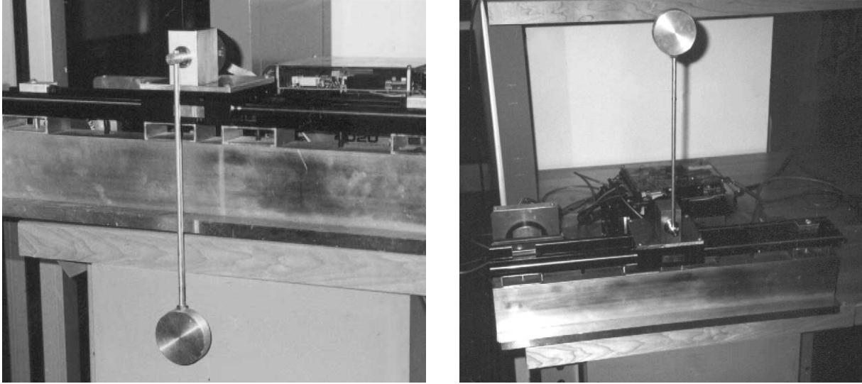
Figure 3.3: Photographs of the Pendulum Cart with pendulum down (left) and up (right).
