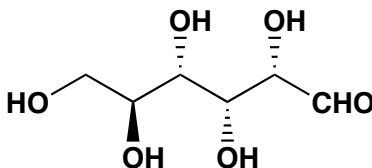
L-Glucose
