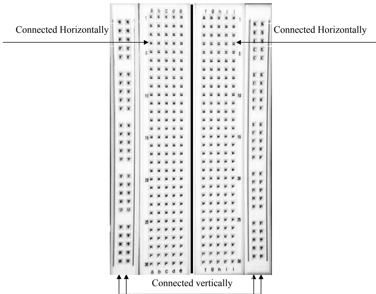
Figure 7 Internal connections of a protoboard.
