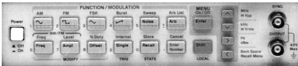
Figure 6 The HP33120A Function Generator Control Panel
