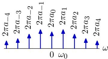
Fourier Transform
