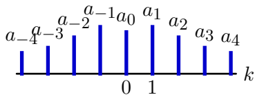
Fourier Series
