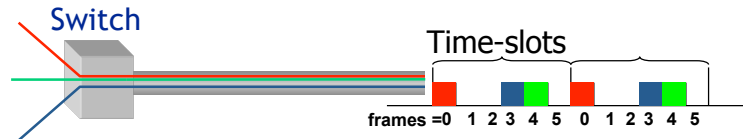
Figure 16-5: Circuit switching with Time Division Multiplexing (TDM). Each color is a different conversation and there are a maximum of N = 6 concurrent communications on the link in this picture. Each communication (color) is sent in a fixed time-slot, modulo N .
