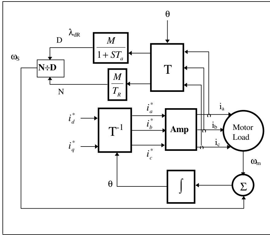
Figure 16: Field Oriented Controller
