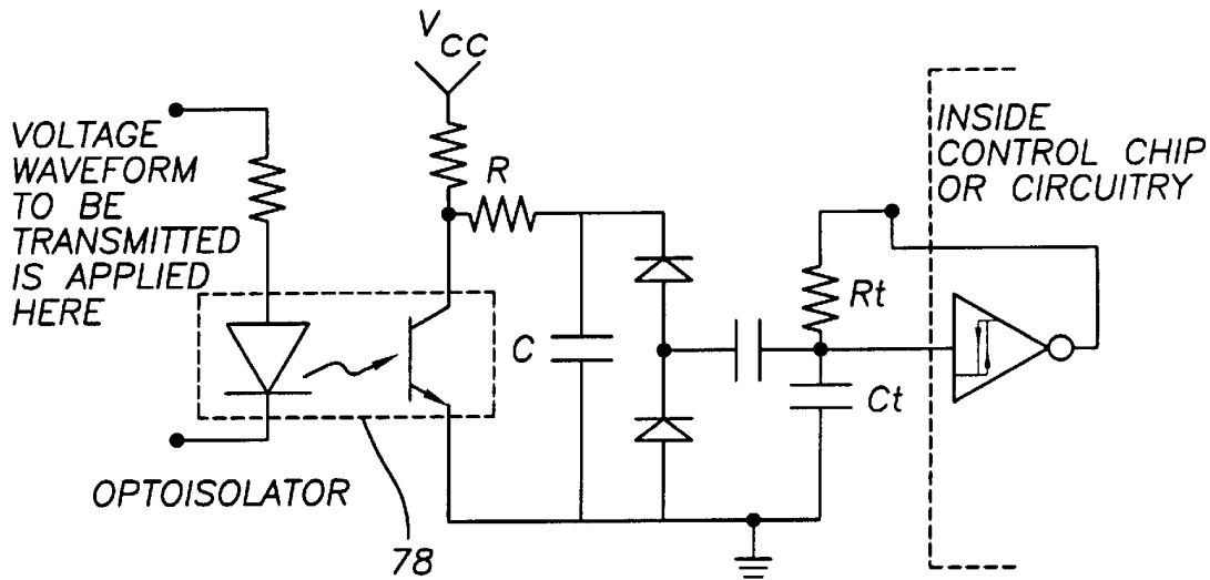
FIG. 7b MODULATION CIRCUITS.
