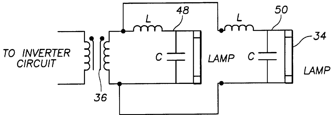
FIG. 6a SAMPLE LOAD CONFIGURITIONS.
