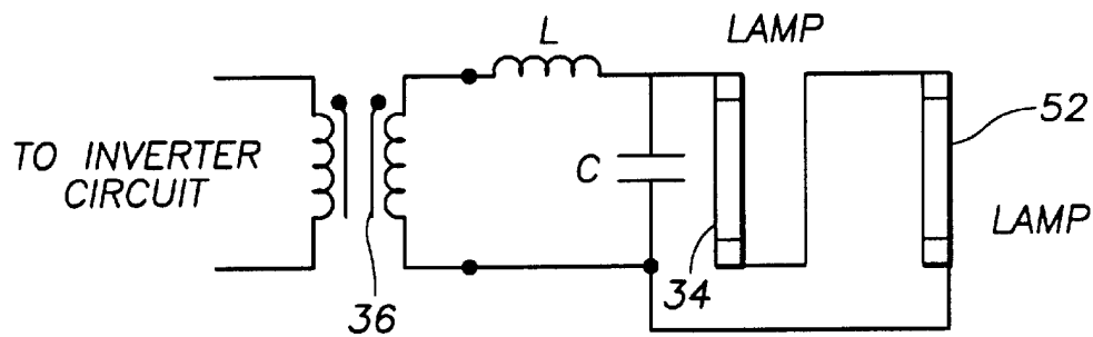
FIG. 6b SAMPLE LOAD CONFIGURITIONS.
