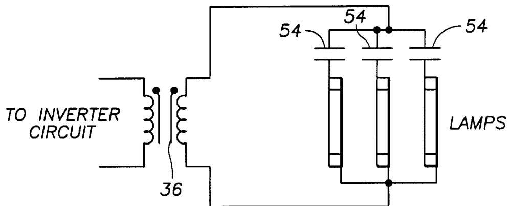
FIG. 6c SAMPLE LOAD CONFIGURITIONS.
