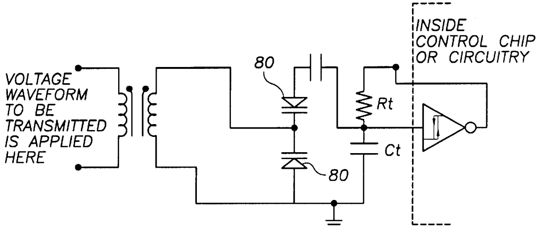
FIG. 7c MODULATION CIRCUITS.
