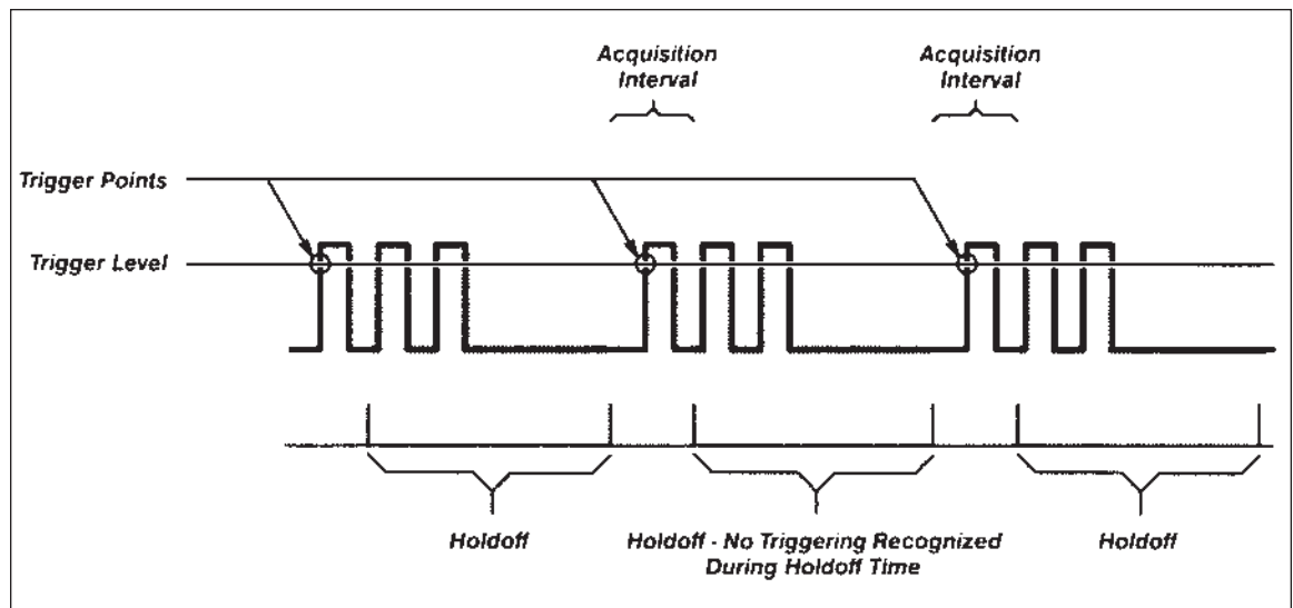
Figure 36. Trigger holdoff.
