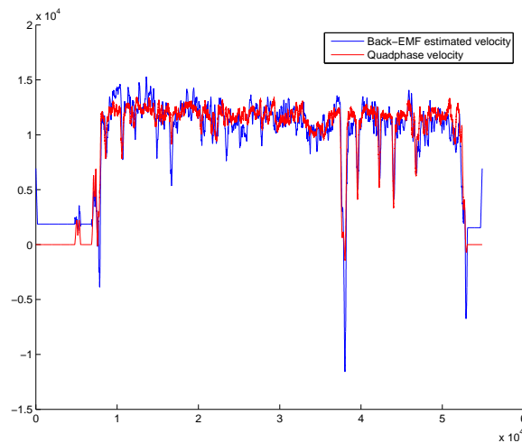
Figure 12: Estimating velocity from current sense. Using Equation 17, we can estimate back EMF (and thus velocity) using the motor's current and applied voltage.
