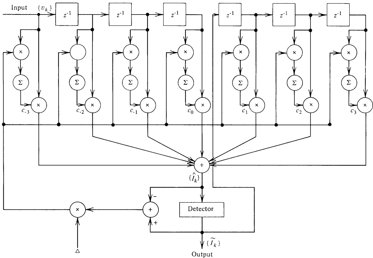
Fig. 10. Decision-feedback equalizer.
