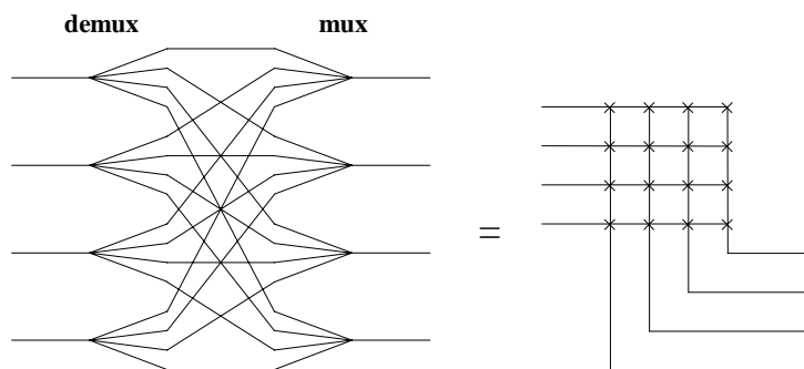
(c) Demux–mux implementation, usually drawn as a crossbar
