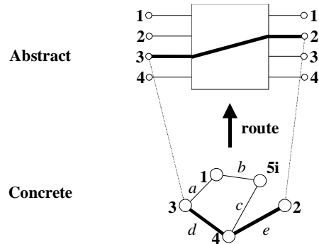
Fig. 8. Composing switches in a mesh.
