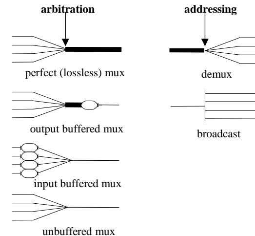
Fig. 1. Multiplexers and demultiplexers. Traffic flows from left to right. Fatter lines are faster channels.
