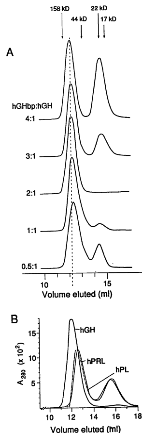
Fig. 3. (A) Gel filtration chromatography of a various ratios of hGHbp to hGH corresponding to 4:1, 3:1, 2:1, 1:1, and 0.5:1 (top to bottom tracings). The concentrations of hGH (fixed at 10 \mu\text{M} except at 1:1 and 0.5:1 ratios, where hGH was 20 \mu\text{M} and 40 \mu\text{M} , respectively) and hGHbp in each mixture were determined by absorbance at 280 nm (6). Protein mixtures were equilibrated for 15 minutes at 25°C in 20 mM tris (pH 7.5), 100 mM NaCl. Samples (100 \mu\text{l} ) were applied to a Superose 12 FPLC column (Pharmacia) and eluted with the same buffer at 0.35 ml/min. Peaks were monitored for absorbance at 280 nm. (B) Gel filtration chromatography of a 2:1 ratio of the hGHbp to hGH (—) and variants of hPRL (-----) or hPL (.....) that were engineered to bind to the hGHbp (8, 9).
