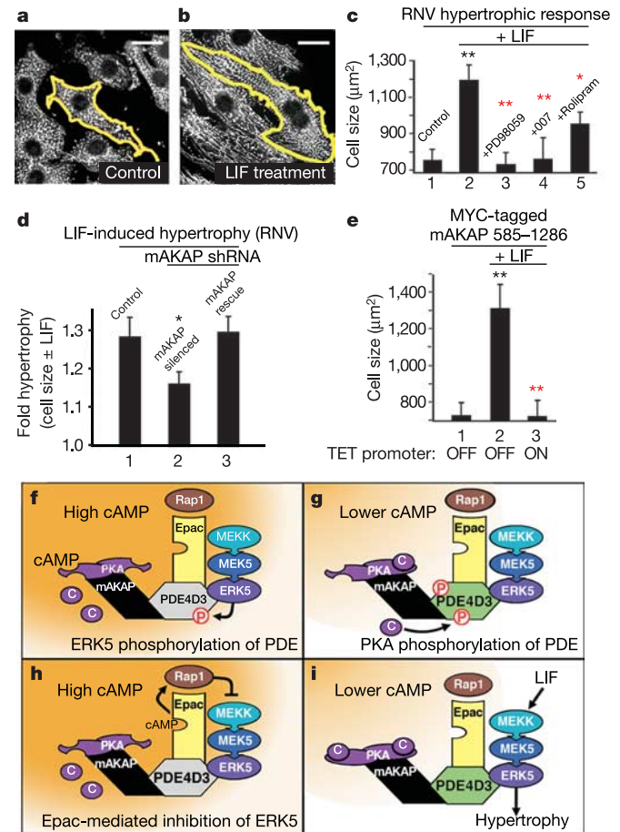
Figure 3 | The mAKAP complex facilitates cytokine-induced cardiac hypertrophy. a–c , Leukaemia inhibitory factor (LIF) induces changes in RNV size. The outline of a rat neonatal ventriculocyte from control ( a ) and LIF-treated ( b ) samples is presented. Scale bar, 20 \mu m. c , Quantification of cell size in control RNVs (lane 1, n = 11 ) and LIF-treated RNVs (lane 2 ( n = 11 ) and lanes 3–5). Pharmacological manipulation of ERK5 (PD98059, n = 4 ), Epac1 (007, n = 4 ) or PDE4 (rolipram, n = 7 ) activity is indicated. d , Expression of mAKAP was suppressed by RNA interference. Quantification of LIF-induced hypertrophy (cell size \pm LIF) in control RNVs (lane 1, n = 12 ), mAKAP-silenced RNVs (lane 2, n = 19 ) and RNVs rescued with a variant of mAKAP resistant to the shRNA (lane 3, n = 13 ). e , Displacement of mAKAP from the nuclear membrane was achieved by overexpression of an mAKAP targeting domain fragment using the TET OFF inducible promoter. Quantification of cell size from control (lane 1, n = 3 ), from LIF-stimulated RNV controls (lane 2, n = 4 ), and from LIF-stimulated cells expressing the mAKAP 585–1286 fragment (lane 3, n = 4 ). P values are indicated by asterisks (black, relative to control; red, relative to sample): single asterisk, P < 0.05 ; two asterisks, P < 0.01 . Error bars in c–e show s.e.m. f–i , Schematics highlighting the main findings of this study. f , ERK5 phosphorylation of PDE4D3 shuts down cAMP metabolism. g , PKA phosphorylation of PDE4D3 enhances cAMP metabolism. h , Activation of Epac mobilizes Rap1 to suppress ERK5 activation. i , Low cAMP represses the Epac-mediated block of ERK5, allowing cardiac hypertrophy.
