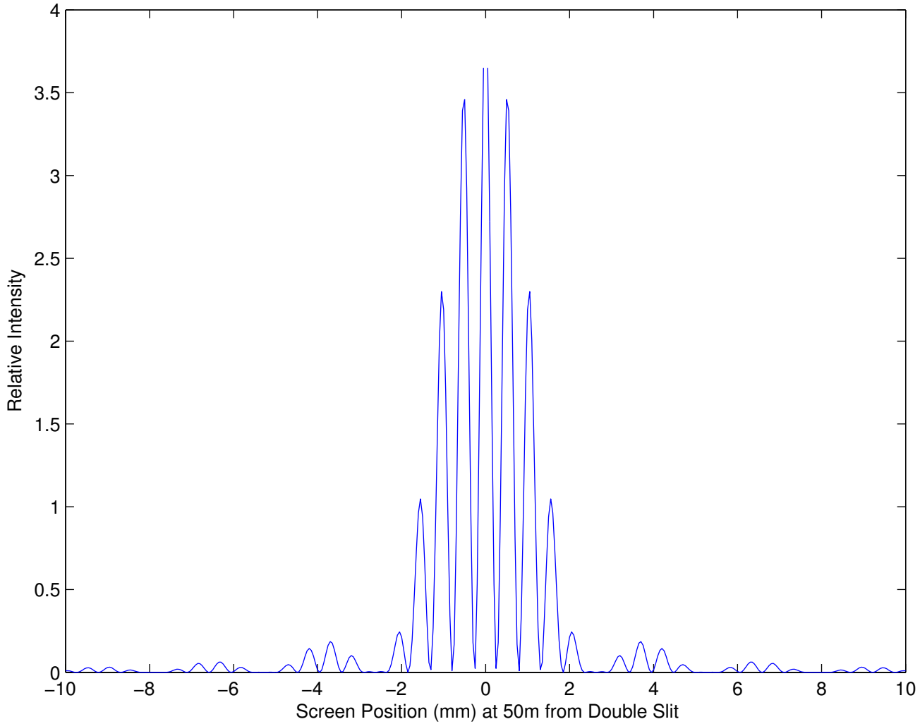
Theoretical Diffraction from a Double Slit, w=120\mu\text{m} , s=600\mu\text{m}
