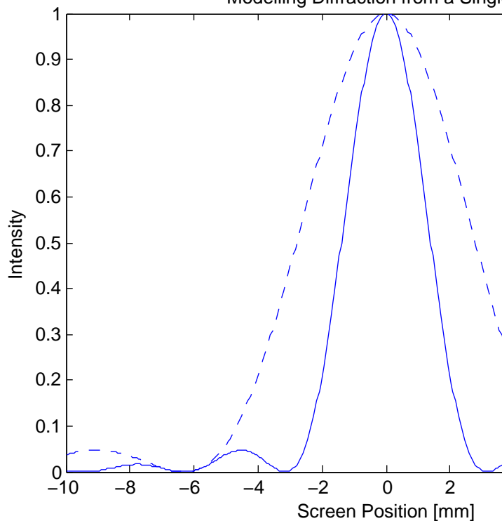
Modelling Diffraction from a Single Slit
