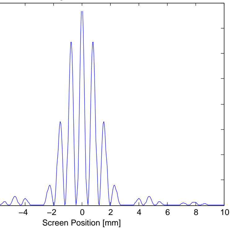
Modelling Two-Slit Diffraction
