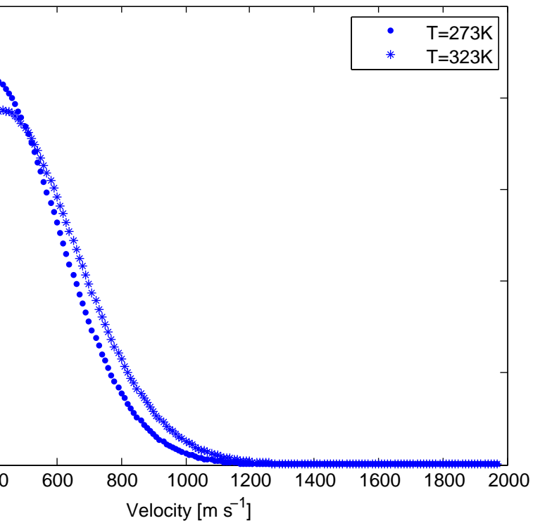
Maxwell-Boltzmann Distribution
