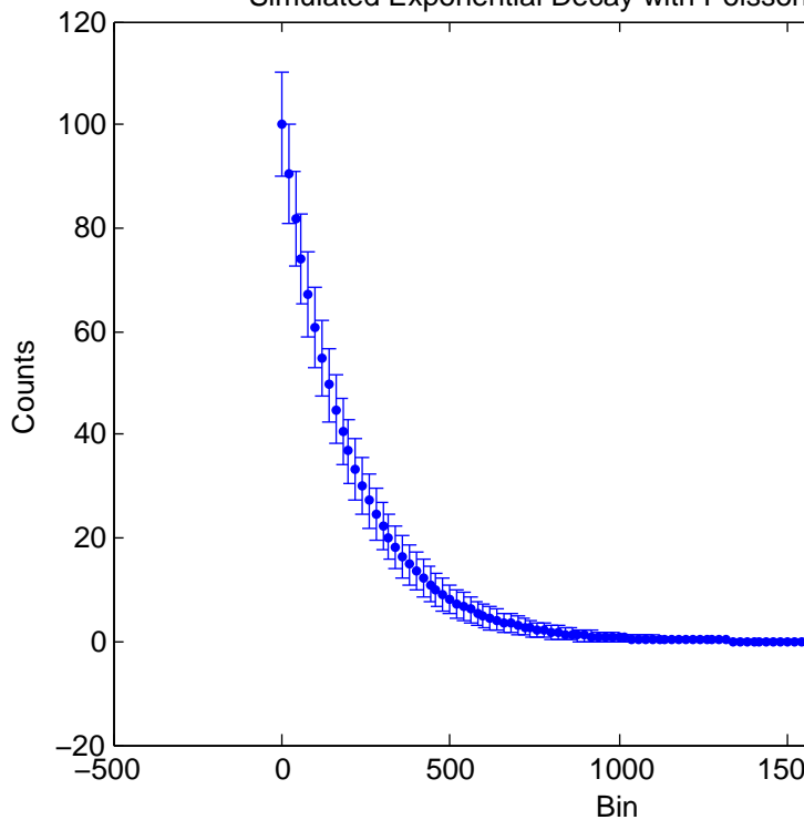
Simulated Exponential Decay with Poisson
