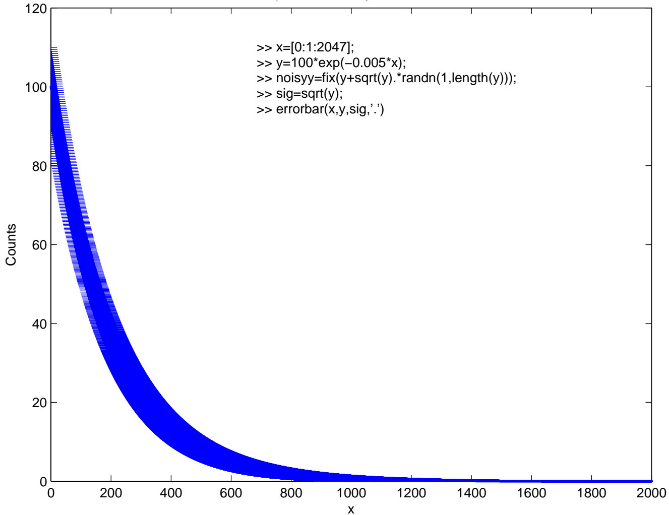
Simulated Exponential Decay with Poisson Statistics
