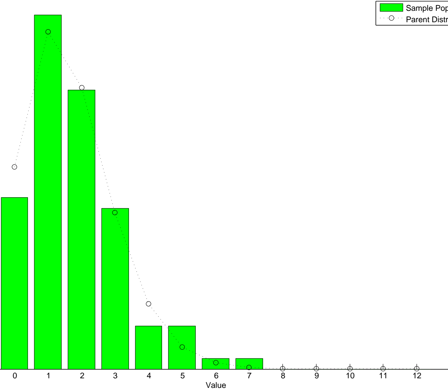
Sample and Parent Distributions – POISSON – \mu=1.67
