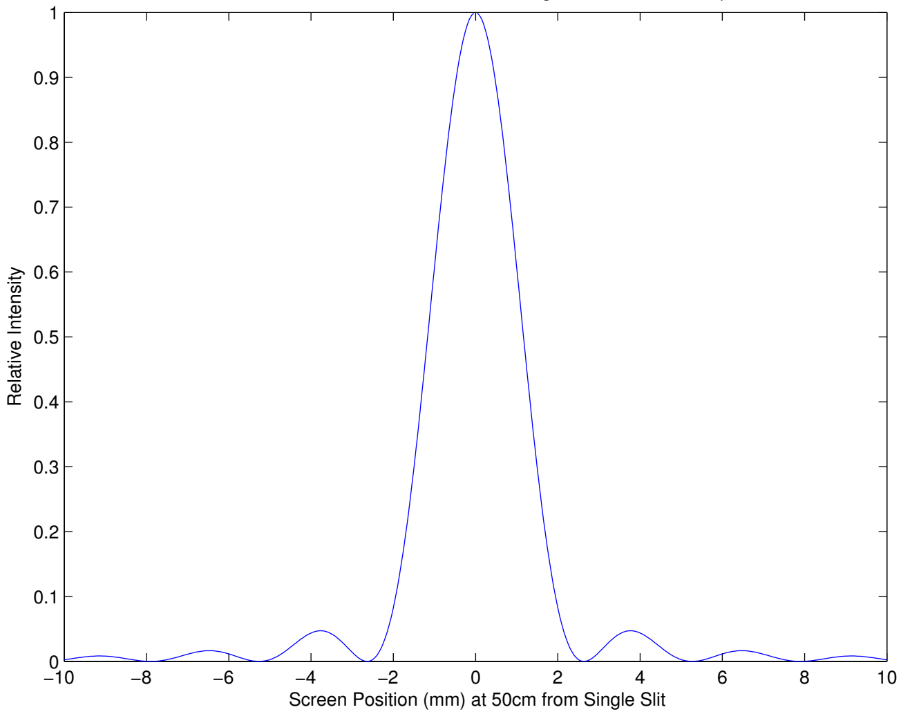
Theoretical Diffraction Pattern from a Single Slit of Width = 120\mu\text{m}
