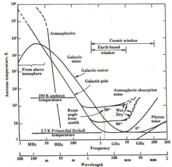
Fig. 8-6. Antenna sky noise temperature as a function of frequency and angle from zenith. A beam angle (HPBW) of less than a few degrees and 100 percent beam efficiency are assumed. (After Kraus and Ko, 1957, cosmic noise between 10 MHz and 1 GHz; Penzias and Wilson, 1965, cosmic noise above 1 GHz; Croom, 1964, atmospheric noise; CCIR, 1964, atmospheric; and Radio Astronomy Explorer Satellite RAE-2, Novaco and Brown, cosmic noise below 10 MHz.)
