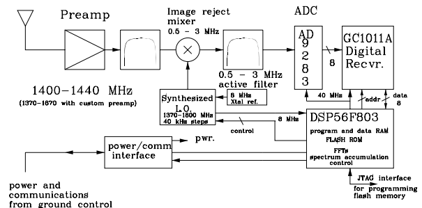
Digital Receiver for SRT seer feb 2002 \mri\rdtdig
