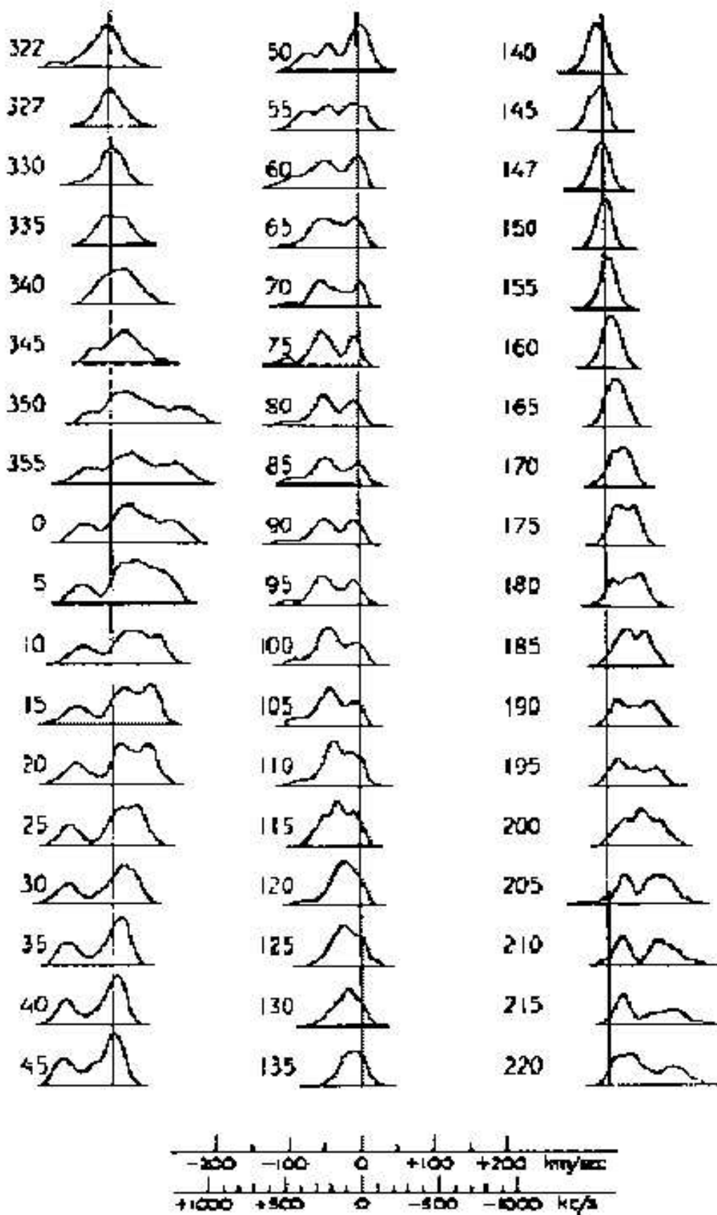
FIG. 7. Survey of hydrogen line profiles at various galactic longitudes. (from H.C. van de Hulst et. al. Bull. of the Astron. Inst. of the Netherlands, XII, 117, May 14, 1954) Note: Pictures are reversed from our images and longitude is given in the old system ( l^I, b^I ). l^{II} = l^I + 32.31^\circ
