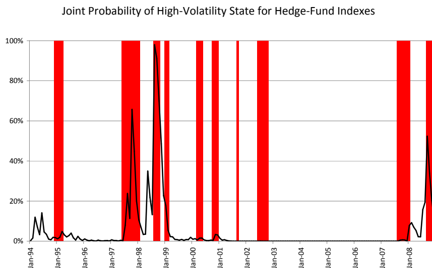
Figure A.2: The joint probability of being in the high-volatility state for the monthly return indexes of Global Macro, Long/Short Equity, Illiquid, and Liquid hedge funds from January 1994 to December 2008. Red vertical bars represent financial crises.
