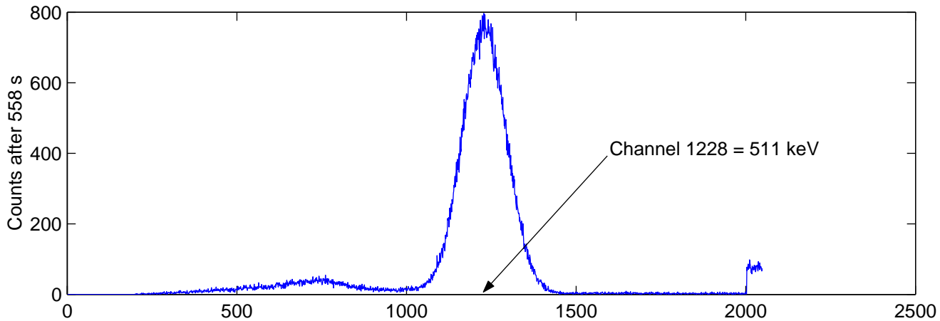
Coincident counts for recoil electron
