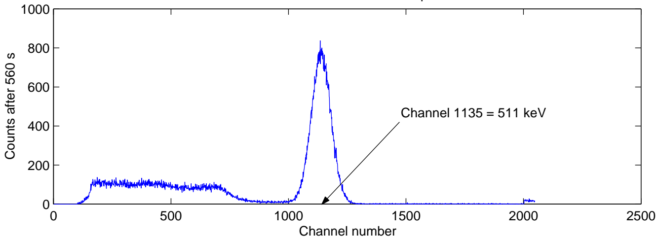
Coincident counts for scattered photon
