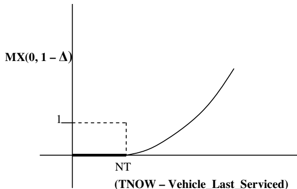
Figure. 14. MX(0, 1 - \Delta)
