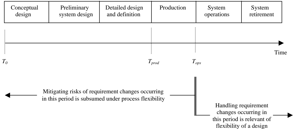
Fig. 7. Time frame attached to a system's life cycle, and time periods associated with process flexibility versus flexibility of a design.
