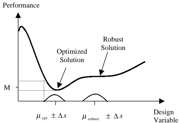
Fig. 4. Type II robust design: Developing flexible solutions. Adapted from [7]. Variation of the design parameter around \mu_{opt} causes greater variation in the performance than when the design parameter is set to \mu_{robust} .
