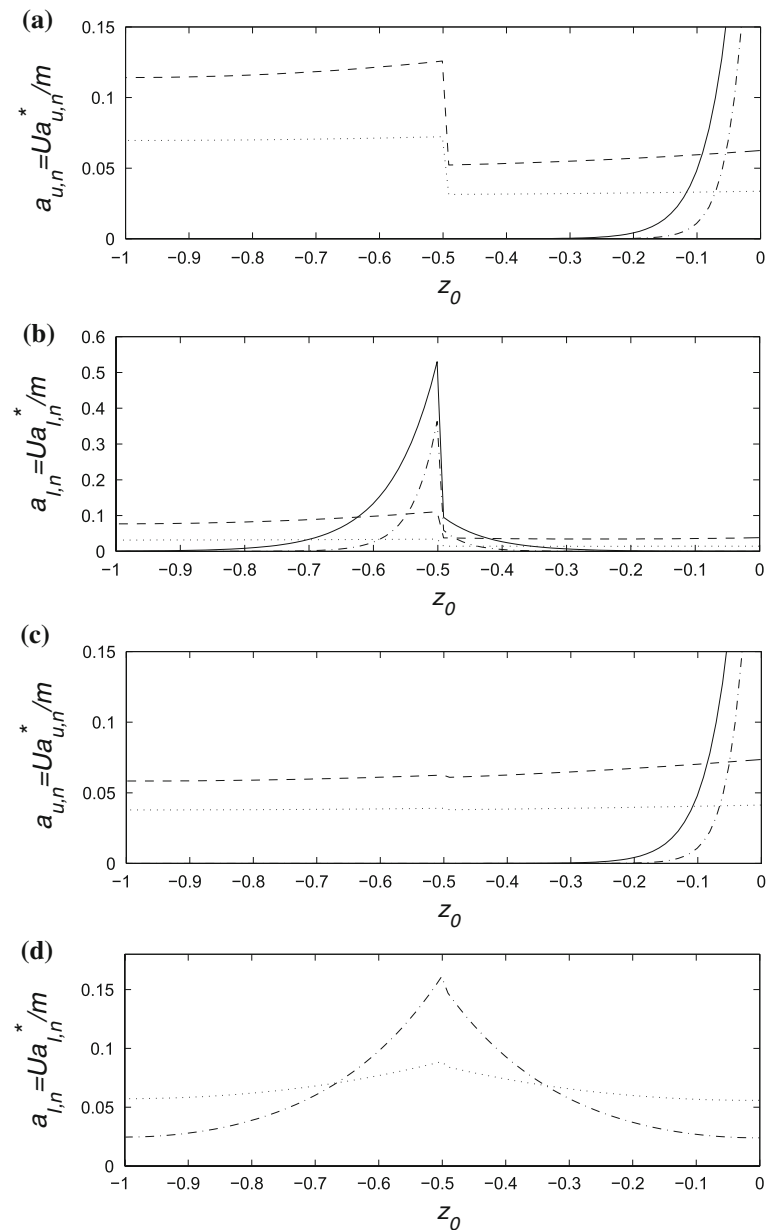
Fig. 6 Far-field wave amplitudes a_{u,n} , a_{\ell,n} , as functions of z_0 for \mathcal{F} = 0.03 , \tau = 0.1 , h = 0.5 , and a, b \mathcal{R} = 0.2 ; c, d \mathcal{R} = 0.95 . In Figs. a, c for a_{u,n} : a_{u,1} —; a_{u,2} - - -; a_{u,3} - · - ·; and a_{u,4} · · · ·. In Figs. b, d for a_{\ell,n} : a_{\ell,5} —; a_{\ell,6} - - -; a_{\ell,7} - · - ·; and a_{\ell,8} · · · ·
