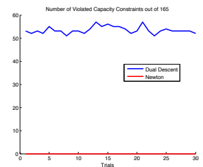
Fig. 6. Number of total capacity constraints violated by two online algorithms over 30 trials with randomly generated capacities each 10-period long.
