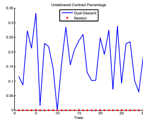
Fig. 5. Percentage of undelivered contracts of two algorithms over 30 trials with randomly generated capacities each 10-period long.
