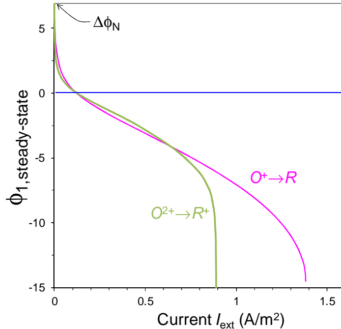
Fig. 3. Steady-state I-V curves for single porous electrode, both for the one-electron reduction of a divalent oxidant (green curves), and for the case of a monovalent oxidant (pink curves).
