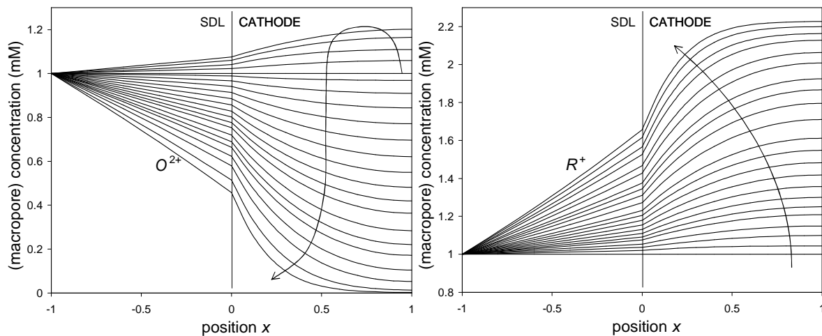
Fig. 4. Concentrations of O^{2+} and R^+ in SDL and in macropores, as function of time after enforcing an external current of I_{\text{ext}}=0.6 \text{ A/m}^2 . For the oxidant (panel left) concentrations first go up, level off, before coming down to settle in the steady-state.
