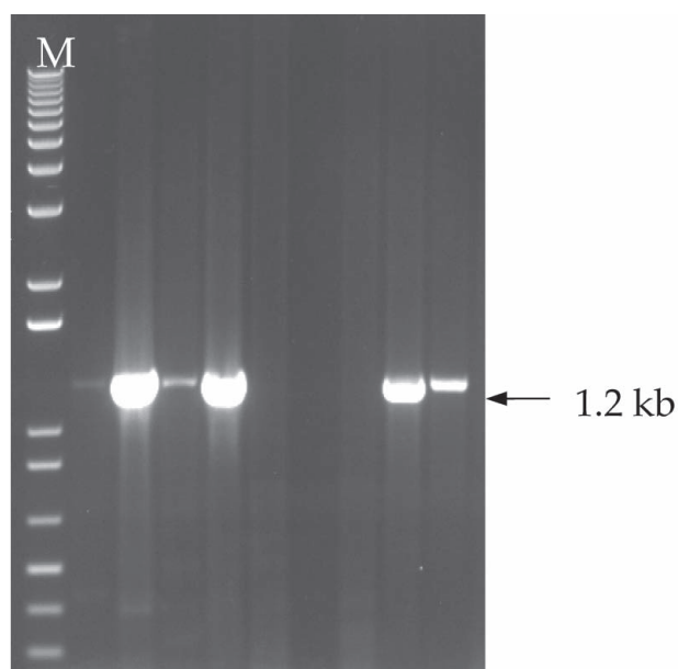
Figure 8. Selection of pMS32 and pMS33 (Arrow indicates the PCR products of ~1.2 kb TpACCase ).
