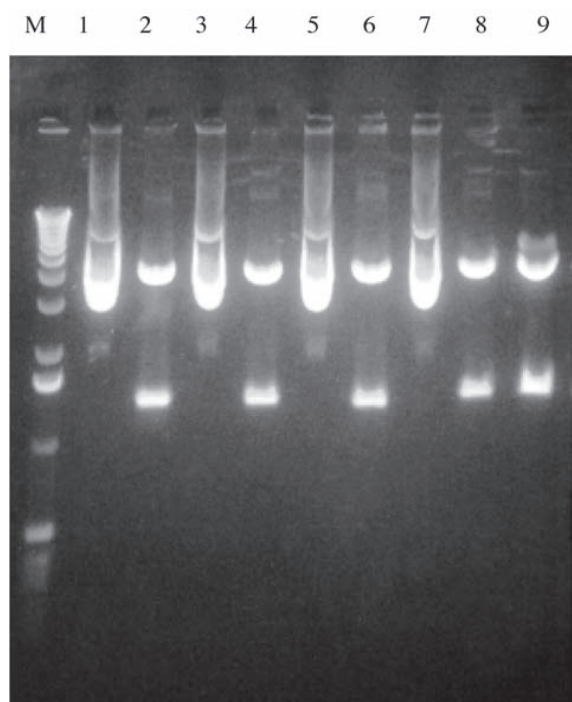
Figure 3. ACCase plasmid digested with EcoR I. All clones examined had inserts of the expected size M: 1 kb marker (Gibco BRL). Lanes 1, 3, 5, 7 undigested plasmid, lanes 2, 4, 6, 8 and 9 digested plasmid with EcoR I.
