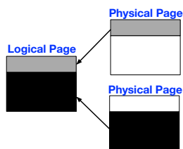
Figure 5: Physical-to-logical page mapping.
