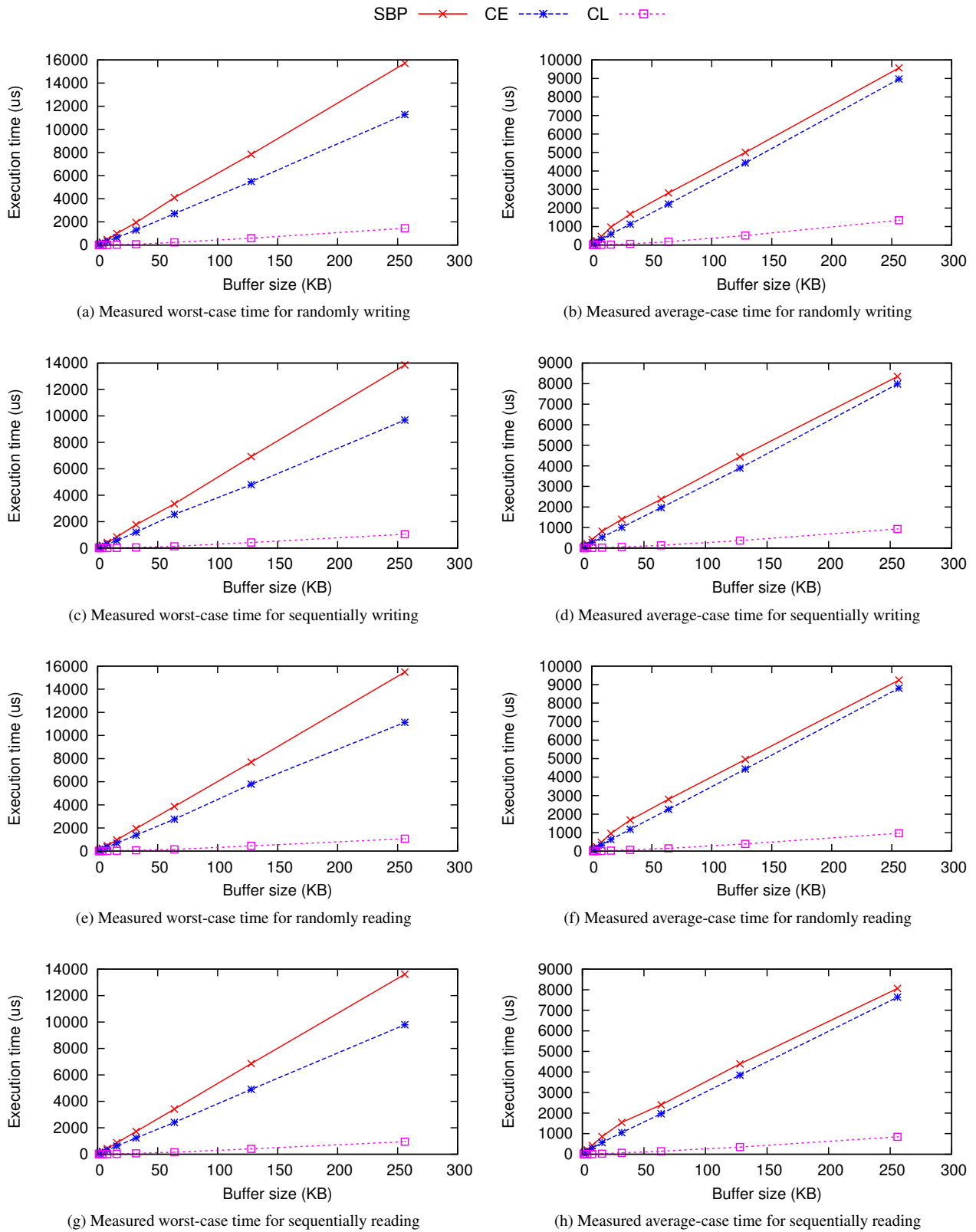
Figure 11: Measured execution data for accessing shared buffers.
