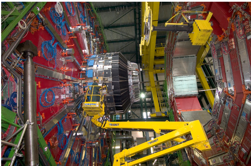
Figure 1. Installation of muon endcap Station 1 on YE+1
