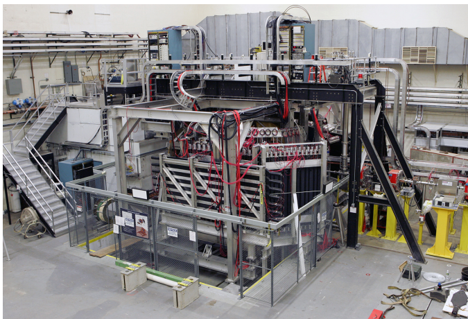
Figure 3. Bates Large Acceptance Spectrometer Toroid (BLAST)
