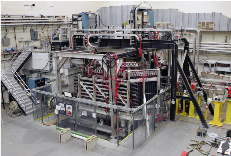
Bates Large Acceptance Spectrometer Toroid (BLAST)
