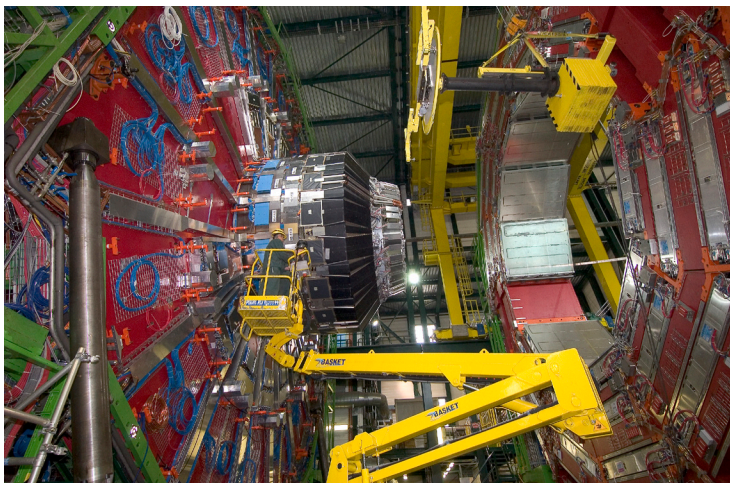
Installation of Muon Endcap Station 1 on YE+1
