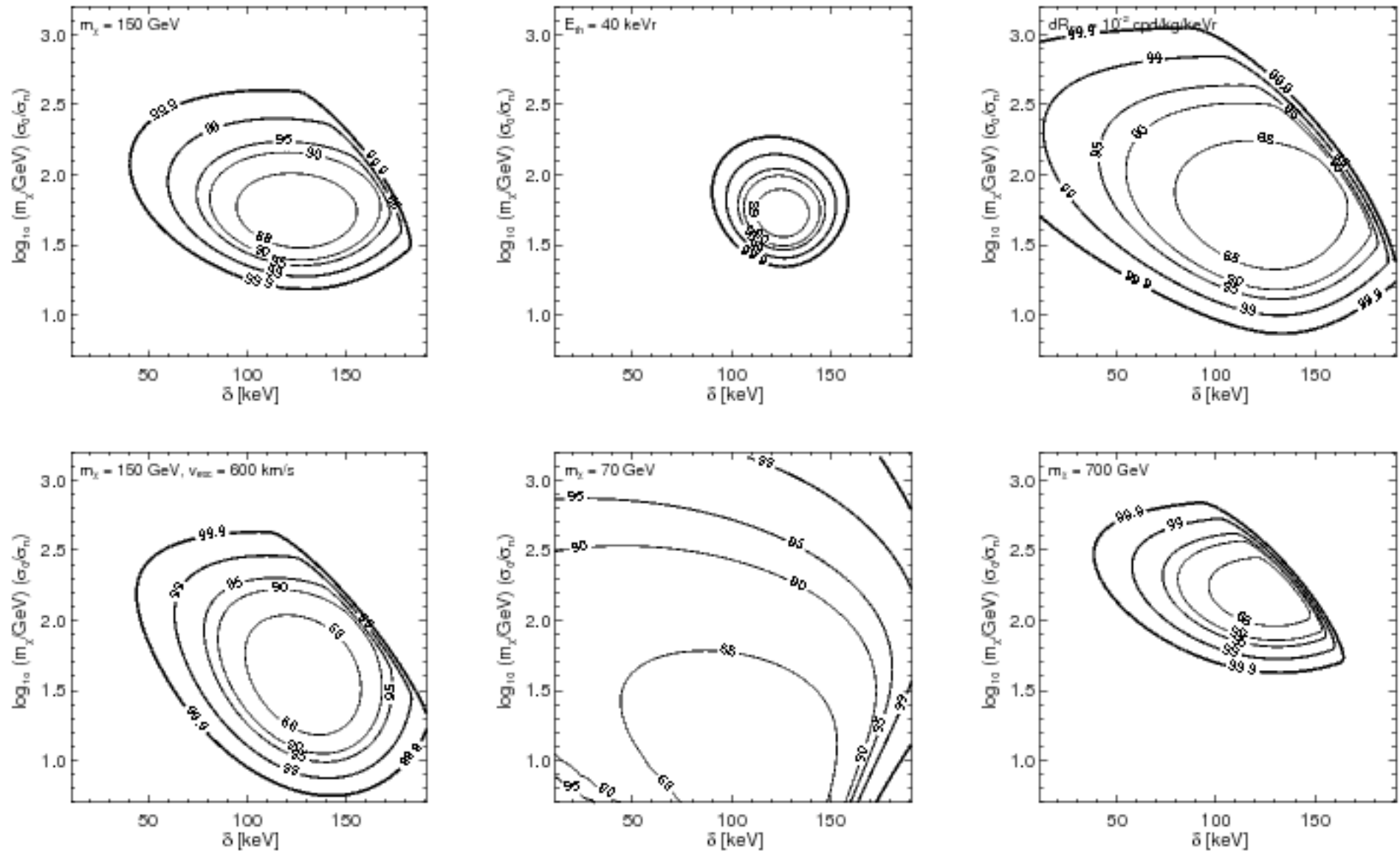
FIG. 9: Confidence levels for determining \delta and m_\chi/\sigma_n , where m_\chi is unknown, with an exposure of 1000 kg · day, taking \sigma_0 = 10^{-40} \text{ cm}^2 . Over most of the parameter space, some value of m_\chi (and therefore \sigma_n ) can be found to produce enough events for the given \delta . However, in the case of large \delta and large m_\chi/\sigma_n , no solution is possible in some cases.
