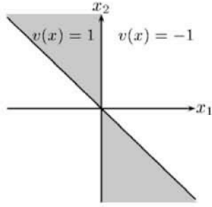
Fig. IV.1. Switching law of Eqn. IV.8
