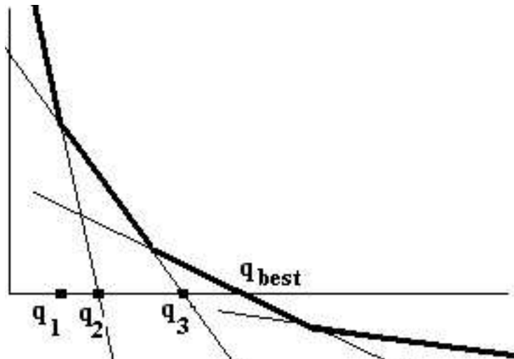
Figure 5: Sequence of q_j 's approaching q_{best}
