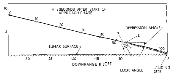
Fig. 1 Approach phase geometry and LM coordinates.
