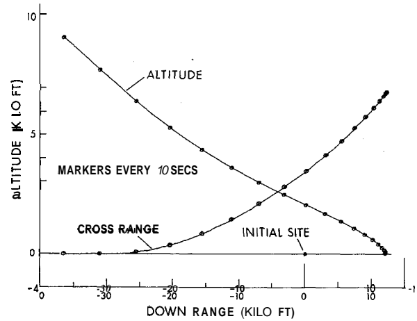
Fig. 11 Elevation and plan views in lunar-fixed coordinates.
