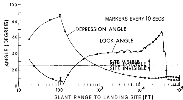
Fig. 15 Look angle and depression to designated site.
