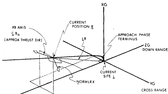
Fig. 10 Geometry pertinent to generation of attitude error signals about the XB axis.
