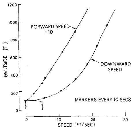
Fig. 13 Forward and downward speeds vs altitude.
