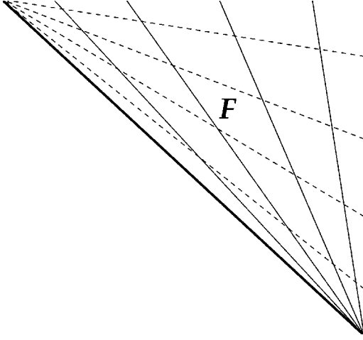
FIG. 1. de Sitter spacetime as covered by the coordinates in Eq. (2). Solid lines are lines of constant r , and dashed lines are lines of constant \eta .
