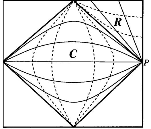
FIG. 2. de Sitter spacetime as covered by the coordinates in Eq. (4). Solid lines are lines of constant r , and dashed lines are lines of constant t . If a (thin-walled) bubble nucleated with center at point P , then region R , the forward light cone of point P , would be contained in the interior of the nucleated bubble. In models of open inflation, region R would contain our observable universe at some time t inside the light cone corresponding to t=0 .
