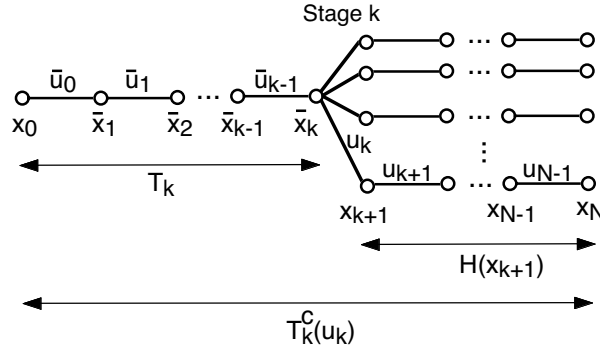
Figure 4.1. Illustration of the rollout algorithm for constrained deterministic DP problems. At stage k , and given the current partial trajectory T_k that starts at x_0 and ends at \bar{x}_k , it considers all possible next states x_{k+1} = f_k(\bar{x}_k, u_k) , u_k \in U_k(\bar{x}_k) , and runs the base policy starting at x_{k+1} . It then finds a control \bar{u}_k \in U_k(\bar{x}_k) such that the corresponding trajectory
