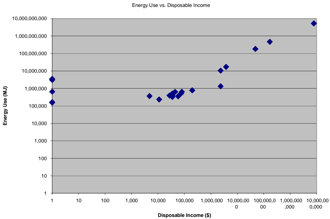
Fig. 2. Energy use versus disposable per capita in the income for 23 different life styles in the U.S. Note that the average energy used U.S. for 1997 was 350 GJ.
