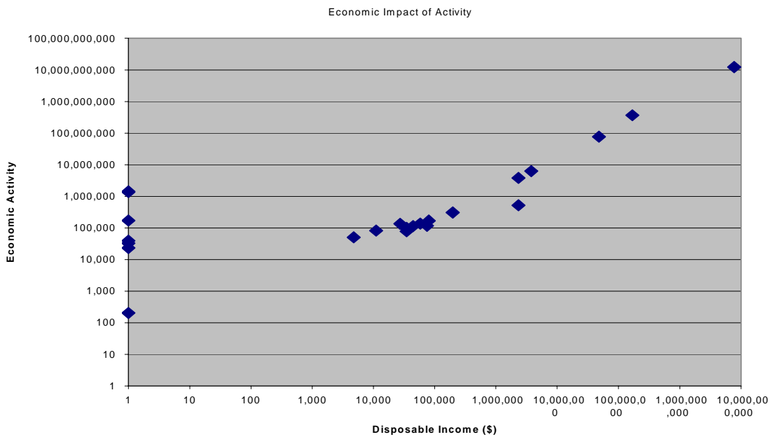
Fig. 4. Economic activity generated by each life style versus disposable income for 23 life styles in the U.S. 1997 data.
