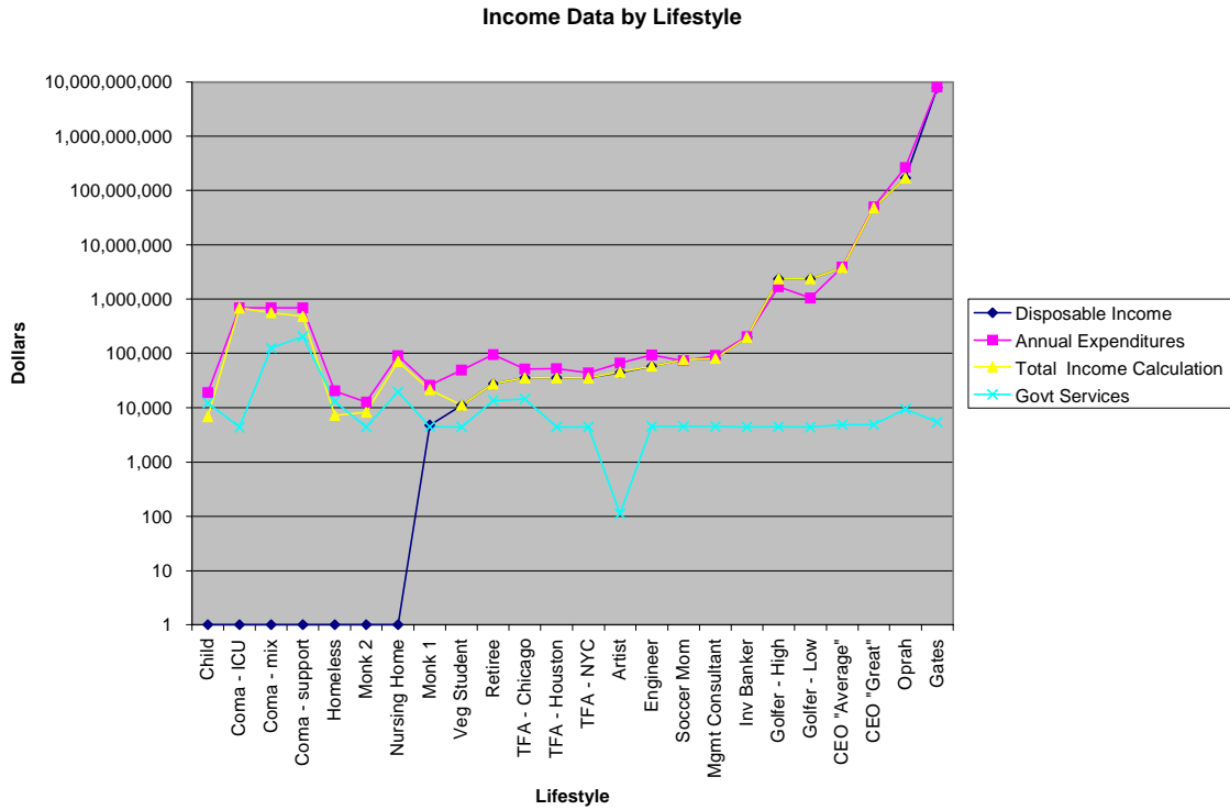
Fig. 1 Disposable Income, Annual Expenditures, Government Services and Total Income calculated for 24 different Life Styles in the United States
