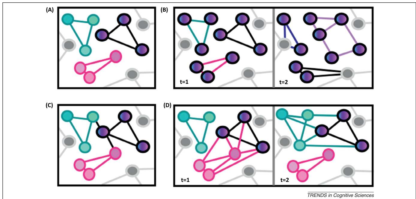
Figure 1. Hypothetical network configurations. A schematic illustration of several hypothetical network configurations [for (B) and (D), we show network configurations at two different time points]. Single-color nodes represent functionally specific brain regions (i.e., regions that are selectively engaged by a particular mental process); multiple-color nodes represent domain-general brain regions (i.e., regions with functionally diverse responses). (A) Two networks comprising functionally specific brain regions and one network comprising domain-general brain regions, with no interaction between the networks. (B) No functionally specific brain regions; all brain regions are domain general but combine in different ways to solve different tasks. (C) Two networks comprising functionally specific brain regions and one network comprising domain-general brain regions, with one node of the latter serving as a 'hub' via which the specialized networks can interact with the domain-general network. (D) Two networks comprising functionally specific brain regions and one network comprising domain-general brain regions. The latter can combine with either of the two specialized networks at different times, thus becoming the 'periphery' of the pink network at t = 1 and of the green network at t = 2 .
