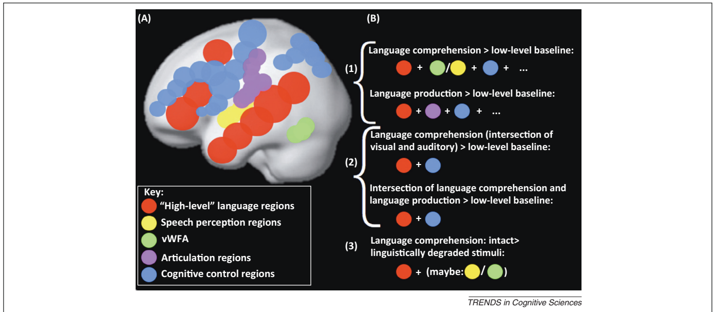
Figure 2. The language network under different definitions. (A) A schematic depiction of five sets of brain regions that are sometimes included in the language network: red, the classic high-level language-processing regions; yellow, speech perception regions; green, visual word-form area; purple, speech articulation regions; and blue, cognitive control regions. (B) A schematic illustration of possible definitions of the language network, ranging from very liberal (1) to more conservative (2 and 3).
